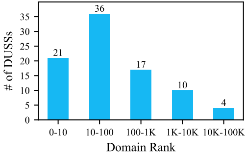
Fig. 3. Domain category ranking statistic of DUSSSs.
