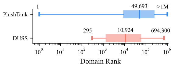
Fig. 6. Domain rank distribution of PhishTank and vulnerable DUSSES.
